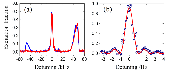
Figure 2. (a) Longitudinal sideband spectra at 173 E_r before (blue line) and after (red line) sideband cooling. The 16-ms sideband cooling reduces the longitudinal temperature from 1.9 \mu\text{K} to 0.8 \mu\text{K} , corresponding to a mean longitudinal motional number \langle n_z \rangle = 0.04 . (b) A typical single-scan, 800-ms Rabi spectrum of the ^1S_0 - ^3P_0 clock transition; the red line is a free-parameter \text{sinc}^2 function fit.
