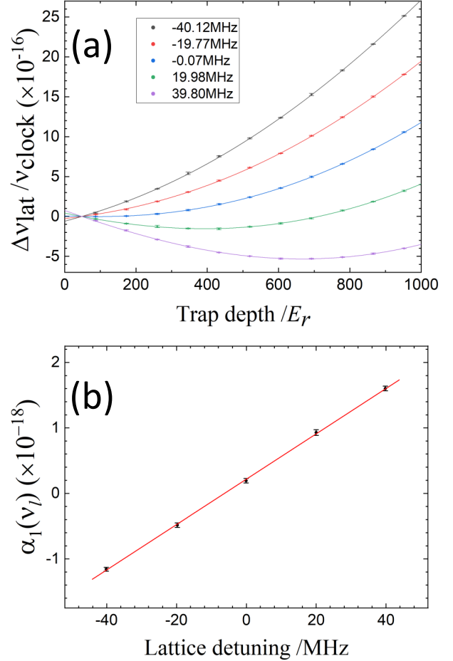
Figure 8. (a) Lattice light shifts as a function of lattice depth. Colored dots represent data sets with distinct detunings of \nu_l relative to the reference frequency 394\,798\,266.9 MHz. Solid lines represent global fits with equation (4). (b) Coefficient \alpha_1 from the global fit as a function of the detuning of \nu_l . The solid line is a linear fit.
