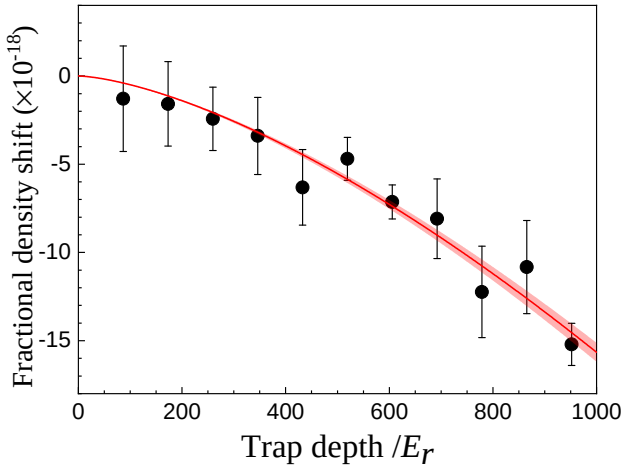
Figure 6. Fractional density shift per N_0 atoms as a function of the lattice trap depth (black dots). These data are fit to \kappa U^{3/2} (red solid line), yielding a scaling factor \kappa = -4.95(16) \times 10^{-22} . The shaded area indicates the 1\sigma confidence band on the fit.
