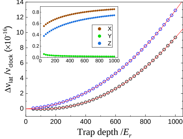
Figure 7. Lattice light shifts (open circles) versus the trap depth, numerically calculated using the BO + WKB model for a radial temperature of T_\rho = \sqrt{U}/3 ( \mu\text{K} ). The lattice light is assumed to be detuned from \nu_{E1} by 3 MHz (black open circles) or -3 MHz (blue open circles). Fractional populations of the axial motional states are assumed to be \langle n_0 \rangle = 0.96 and \langle n_1 \rangle = 0.04 . Each of the two datasets is fitted with a fourth-order polynomial in the form of equation (4) (the red curves). The inset displays the calculated values of X , Y and Z .
